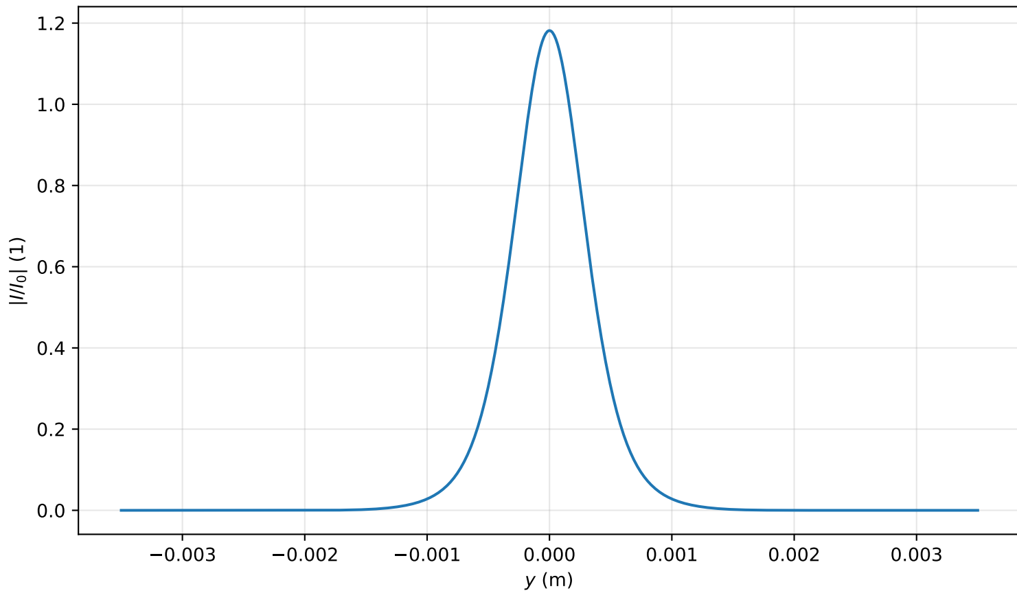
Intensity profile I(x=0, y, z=1.592)/I_0 , P_{in}=0.7P_{cr} , artificial time
